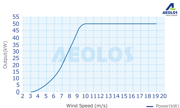
Wind Speed/ Power Curve
