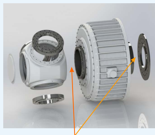
Directly Connection Without Flanges
