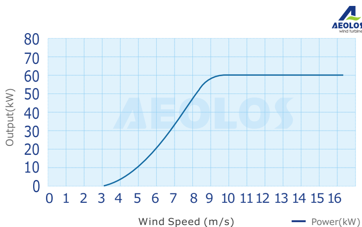
Wind Speed/ Power Curve
